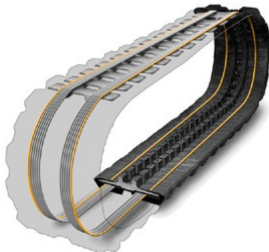
CLOSE-UP OF motiondynamics™ BOBCAT T190 CONTINUOUS WRAP STEEL CABLES:
