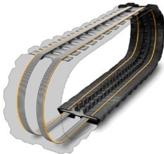
CLOSE-UP OF motiondynamics™ BOBCAT T300 CONTINUOUS WRAP STEEL CABLES:
